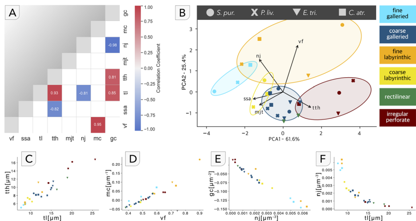
Fig. 5 (A) Matrix of correlation pairwise correlation coefficients for descriptors of the 6 major stereom subtypes found in the coronal plates of four species of sea urchins. vf: mineral volume fraction [a.u.]; ssa: specific surface area [ \text{m}^2 \text{cm}^{-3} ]; tth: mean trabecular thickness [ \mu\text{m} ]; tl: mean trabecular length [ \mu\text{m} ]; mjt: mean joint type as defined in the skin library; nj: number density of trabecular junctions [ \mu\text{m}^{-3} ]; mc: mean curvature [ \mu\text{m}^{-1} ]; gc: gaussian curvature [ \mu\text{m}^{-2} ]. (B) Biplot of principle component analysis of morphometric descriptors for 6 major stereom subtypes (cyan: fine galieried; blue: coarse galieried; orange: fine labyrinthic; yellow: coarse labyrinthic; green: rectilinear; red: irregular perforated) found in the coronal plates of four species of sea urchins (circle: S. pur. ; cross: P. liv. ; triangle: E. tri. ; square: C. atr. ). Loadings for the descriptors vf, ssa, tth, mjt, and nj are indicated (black arrows). The confidence ellipses are drawn with radii of 1.6 standard deviations and are shaded according to the color of the stereom subtype they represent. The associated scree plot is presented in Fig. S13.† (C–F) Scatterplots of the strongly correlated descriptor pairs trabecular thickness and length (C), mean curvature and volume fraction (D), gaussian curvature and number density of trabecular junctions (E), and number density of trabecular junctions and mean trabecular length (F).
