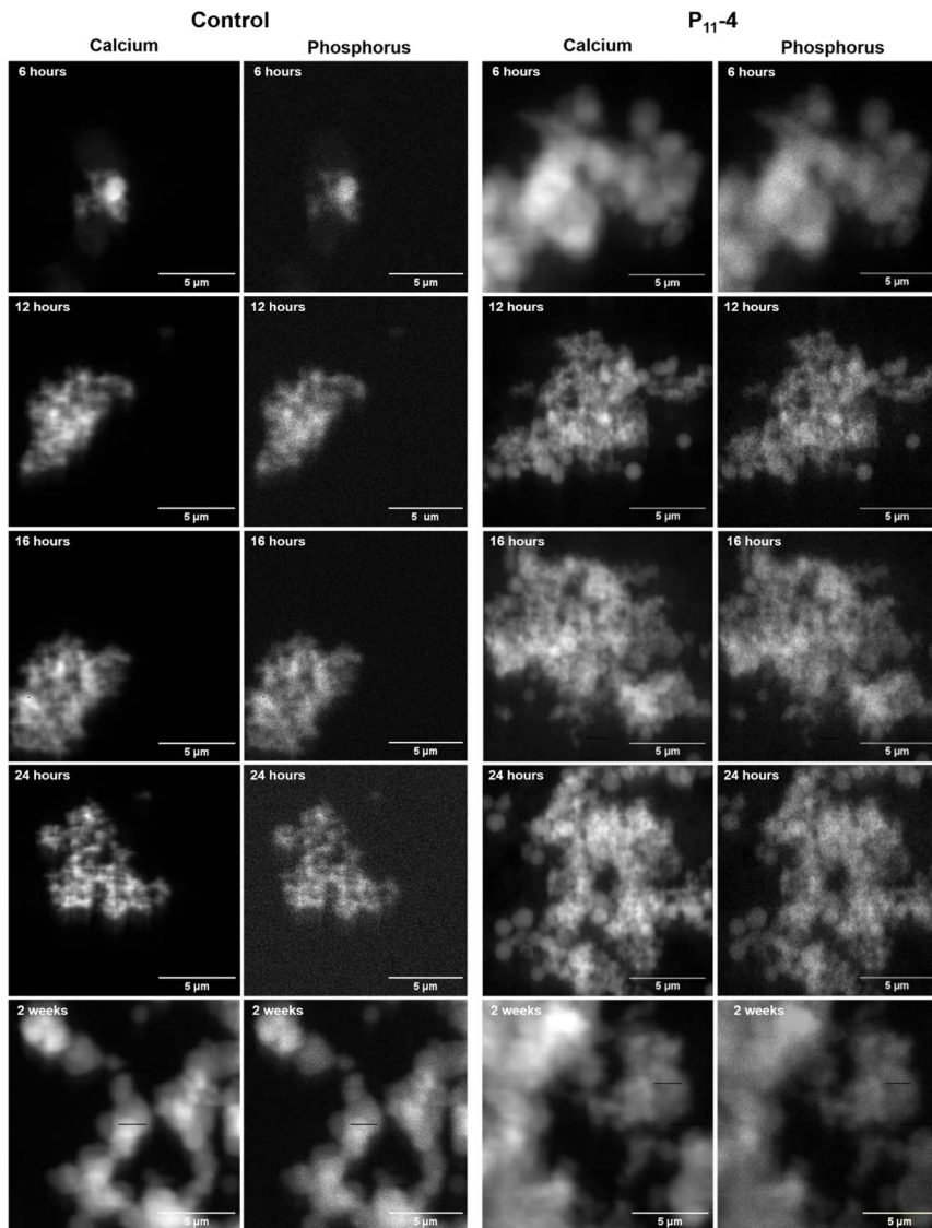
Fig. 3 Typical calcium and phosphorus elemental maps at different time points (6 hours, 12 hours, 16 hours, 24 hours and 2 weeks) comparing the control to the mapped SiN windows with deposited P_{11-4} , extracted using n-XRF mapping on the I14 beamline. These maps depict the morphology of the formed calcium phosphate structures. The area shown is 15\ \mu\text{m} \times 15\ \mu\text{m} , with a step size of 50\ \text{nm} .
