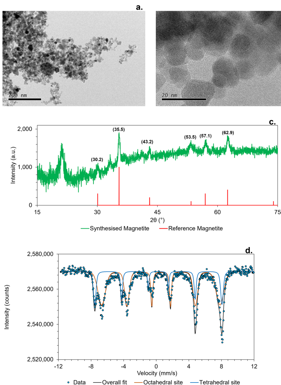
Fig. 1 Characterization of synthesised MNPs. a) Transmission Electron Microscopy (TEM) of MNPs at 200 nm scale and b) at 20 nm scale, c) depicts X-Ray Diffraction (XRD) reflections of MNPs with the synthesised sample in green and a reference magnetite reference in red. XRD measurements were obtained using the Cu radiation ( \lambda = 1.5406 \text{ \AA} ). d) Mössbauer spectra of synthesised MNPs at room temperature (295 K).
