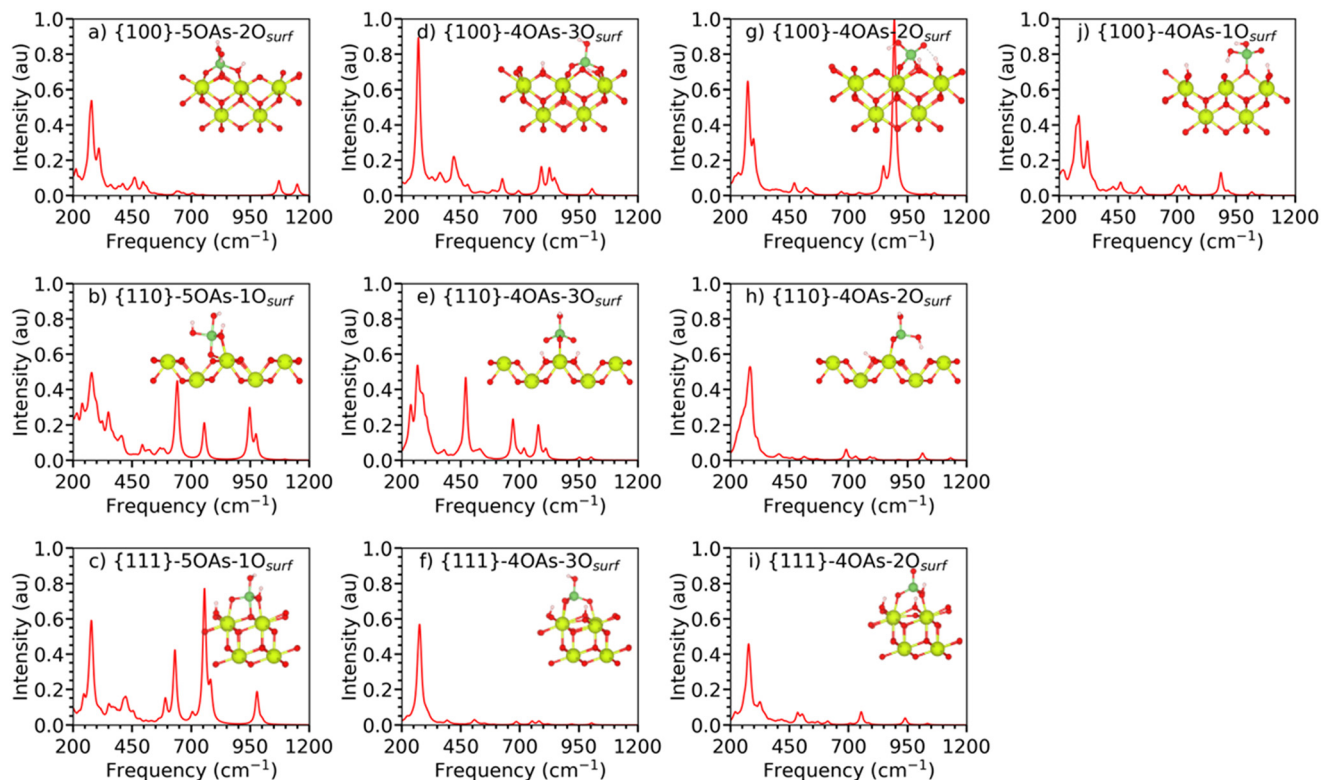
Fig. 3 Simulated IR spectra of arsenate species adsorbed onto the {111}, {110}, and {100} stoichiometric surfaces of CeO 2 with different binding modes as shown by the inset structures. The spectra are normalised relative to each other such that the highest absolute intensity across all the spectra is set to unity.
