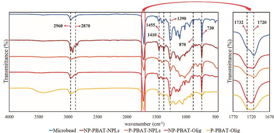
Fig. 2 Infrared spectra of NP- and P-PBAT-NPLs and NP- and P-PBAT-Olig and the initial material (PBAT microbeads).
