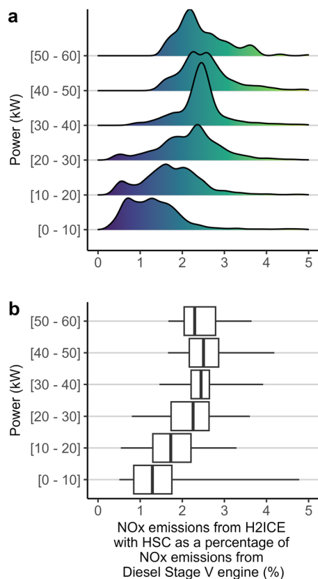
Fig. 4 The difference in instantaneous NO x emissions as a function of power setting between H2ICE with HSC and Stage V diesel engine for the across the NRTC. (a) Shows the distribution as density plots and (b) shows data as a box and whisker plot with median, interquartile and 5th and 95th percentile ranges.
