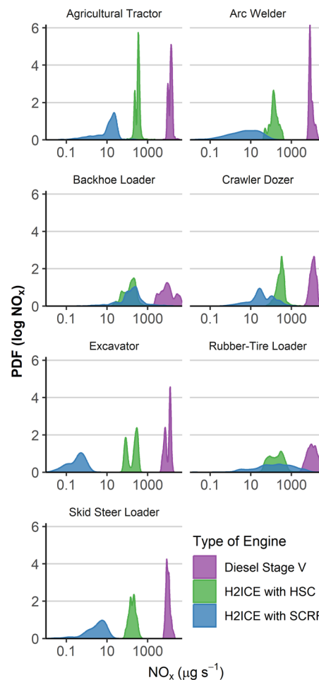
Fig. 5 NO x emissions distribution for the seven applications within the NRTC for (i) diesel Stage V, (ii) H2ICE with hydrogen slip catalyst (HSC), and (iii) H2ICE with selective catalytic reduction and particulate filter (SCRF).
