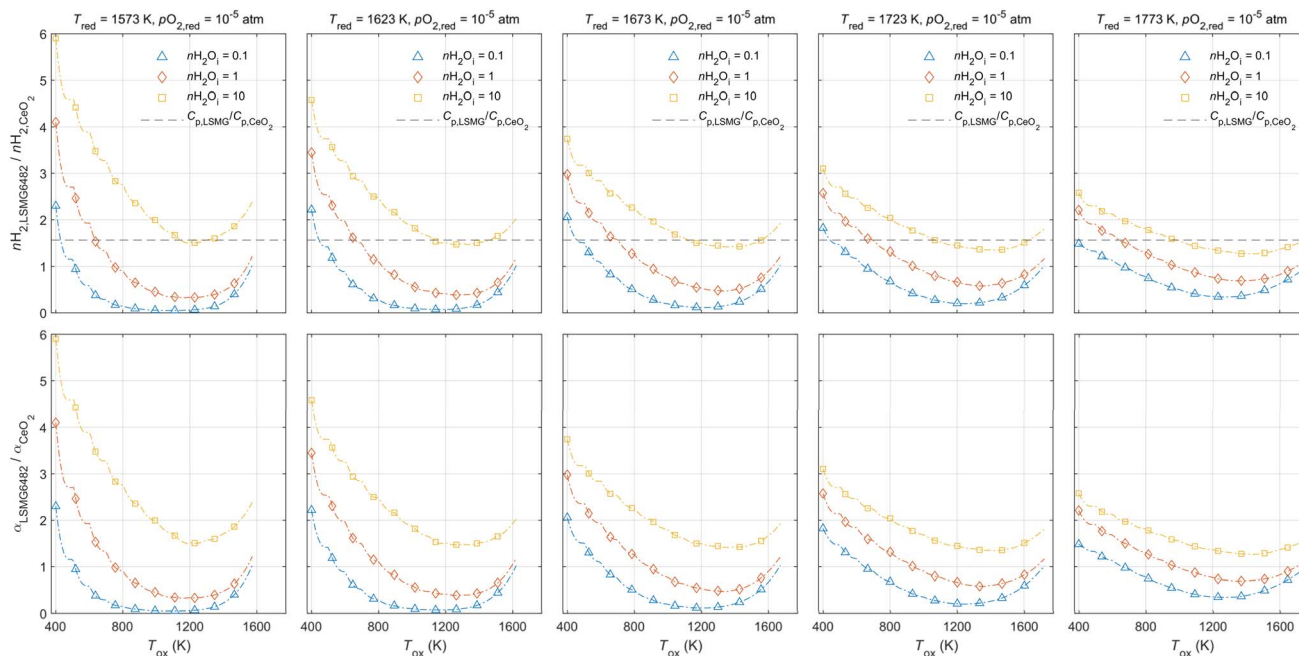
Fig. 10 n\text{H}_{2,\text{LSMG6482}} normalized to that of ceria (top row) for 1573\text{ K} \leq T_{\text{red}} \leq 1773\text{ K} (columns) and varying n\text{H}_2\text{O}_i , noted by different colors and markers. The criterion for thermodynamic advantage over ceria under a given \Delta T , specifically the ratio of specific heat capacities of each solid, is shown by the dashed line. It is assumed here based on specific heat capacity correlations that C_{p,\text{LSMG6482}} and C_{p,\text{ceria}} are equal \sim 94\text{ J mol}^{-1}\text{ K}^{-1} and \sim 60\text{ J mol}^{-1}\text{ K}^{-1} , respectively. 31–33
