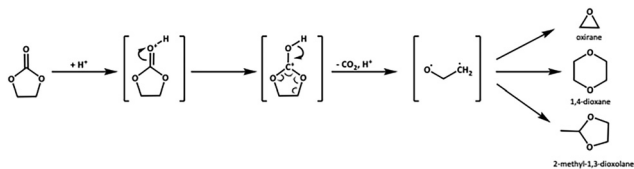
Fig. 5 Proposed reaction scheme for \text{H}^+ -catalyzed decomposition of EC. The reaction branches out after the formation of \text{CO}_2 and \bullet\text{O}-\text{CH}_2-\text{CH}_2\bullet moieties from the ring opening process, to form a series of ether-based molecules and polymers. The scheme shows molecules detected in our experiments only.
