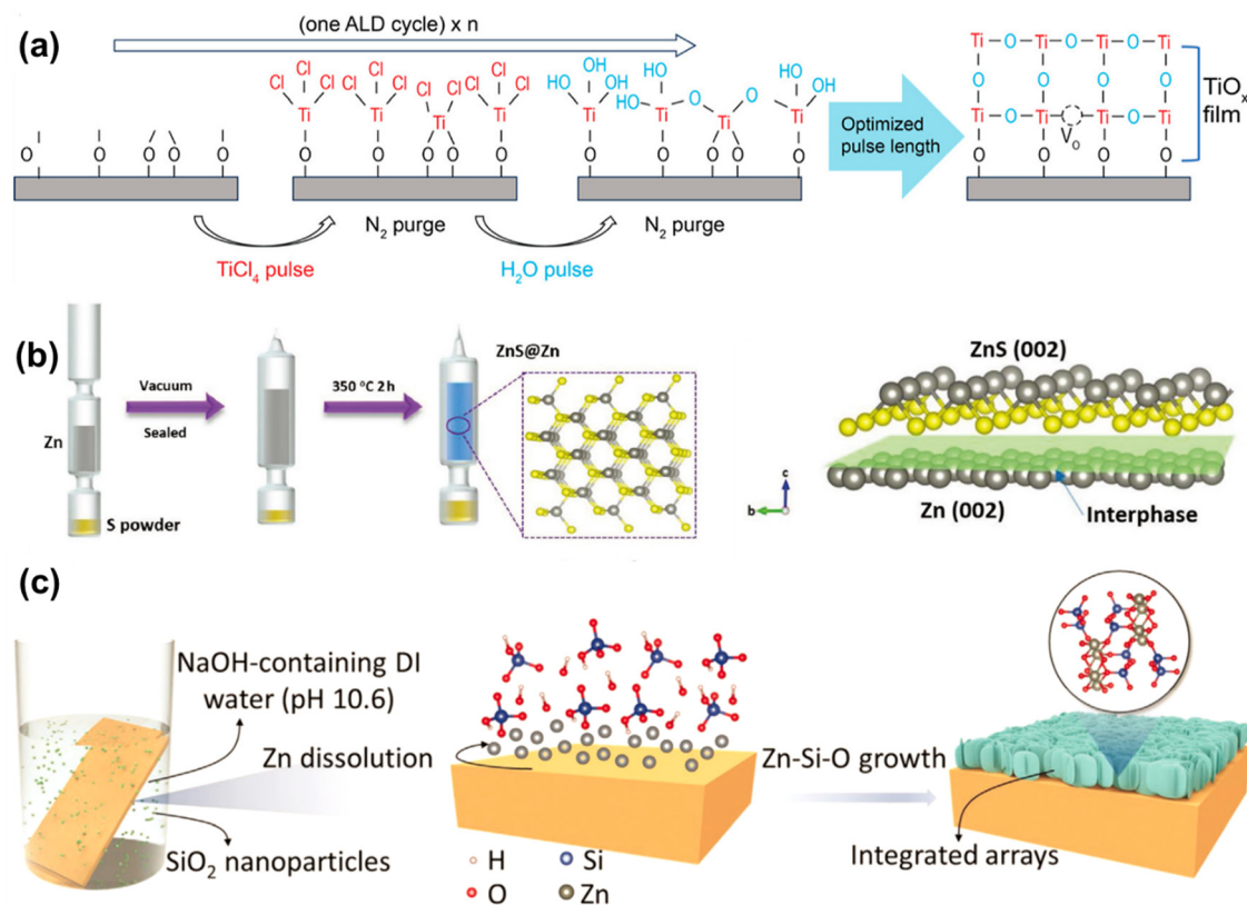
Fig. 9 (a) Illustration of a single ALD cycle with a TiO x coating of thickness of \sim 0.04 nm. Reproduced from ref. 154 with permission from the American Chemical Society, copyright 2024. (b) Schematic of the artificial ZnS layer preparation. Reproduced from ref. 155 with permission from John Wiley & Sons, copyright 2020. (c) Schematic of the procedure for fabricating the Zn@ZSO composite foil. Reproduced from ref. 156 with permission from John Wiley & Sons, copyright 2022.
