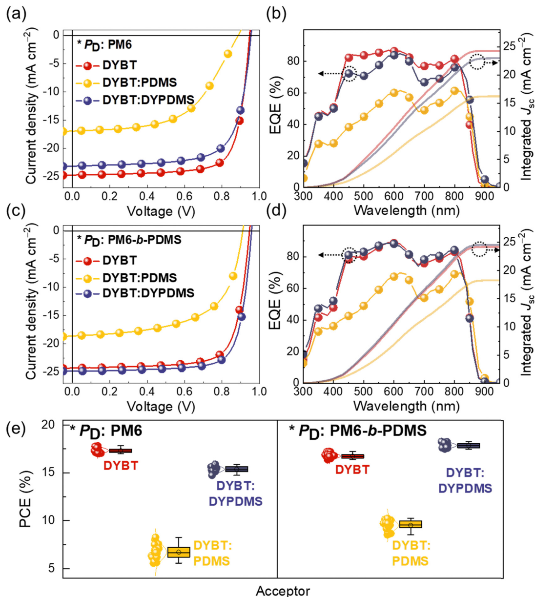
Fig. 3 (a) J-V curves and (b) EQE spectra of PM6:acceptors-based OSCs. (c) J-V curves and (d) EQE spectra of PM6-b-PDMS:acceptors-based OSCs. (e) Gaussian function fitted PCE distributions of the OSCs.
