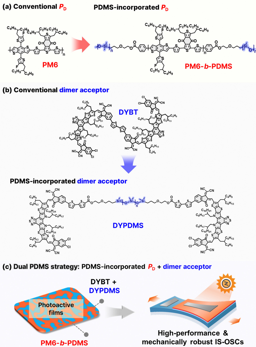
Fig. 1 (a) Chemical structures of conventional (PM6) and PDMS-incorporated P_D s (PM6-b-PDMS). (b) Chemical structures of conventional (DYBT) and PDMS-incorporated dimer acceptors (DYPDMS). (c) Conceptual illustration of the dual PDMS incorporation strategy to achieve enhanced mechanical robustness and photovoltaic performance in IS-OSCs.
