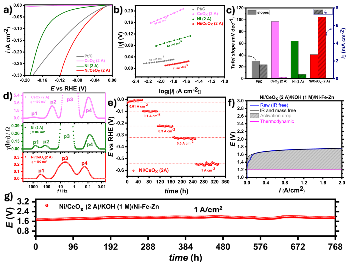
Fig. 3 Electrocatalytic activity of the designed catalysts. (a) HER LSVs, (b) HER Tafel plots, (c) Tafel slopes and exchange current densities of the designed films. (d) DRT analysis for the HER at the designed films. (e) HER chronopotentiogram of Ni/CeO x (2 A) at 20 °C. (f) Deconvoluted LSV and (g) chronopotentiogram at 1 A cm -2 in a 2-electrode electrolysis cell at 60 °C.
