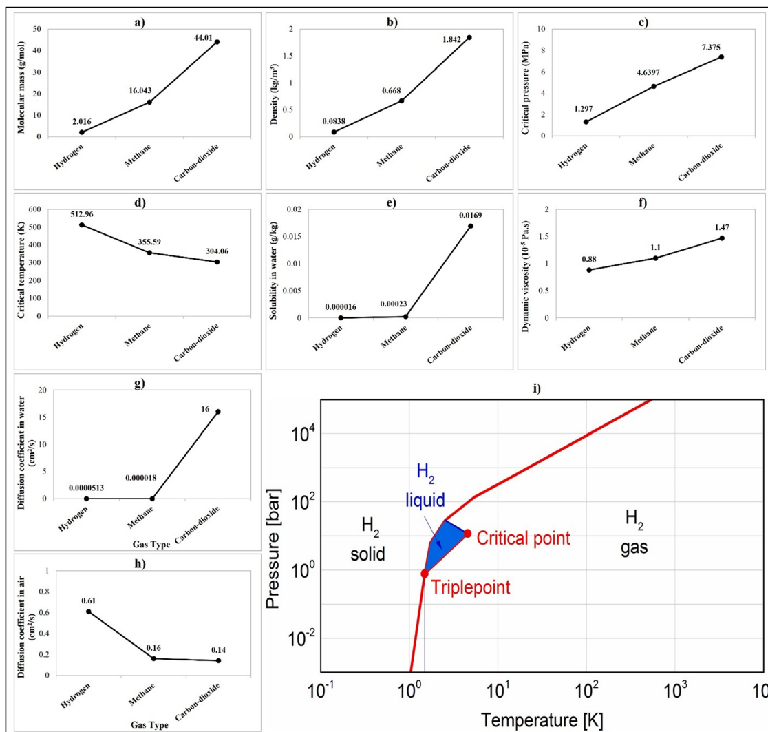
Fig. 5 Hydrogen ( \text{H}_2 ) phase diagram and comparison of physical properties of \text{H}_2 with methane ( \text{CH}_4 ) and carbon dioxide ( \text{CO}_2 ). This figure was modified from ref. 95 and 99, and data are from ref. 100–104. (a)–(h) Comparison of the molecular mass, density (293 K and 0.1 MPa), critical pressure, critical temperature, water solubility, dynamic viscosity (293 K and 0.1 MPa), diffusion coefficient in water, and diffusion coefficient in air for \text{H}_2 , \text{CO}_2 , and \text{CH}_4 . Understanding these physical properties is essential for predicting the thermodynamics and behavior of gas in a respective environment. (i) This figure illustrates how \text{H}_2 changes its physical state under temperature and pressure conditions.
