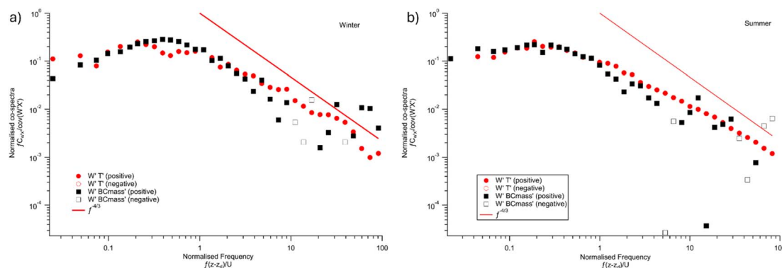
Fig. 1 Co-spectral analysis in winter (194 cases, (a)) and summer (201 cases, (b)) which are binned into 40 evenly spaced bins. BC flux < 0 ng -2 s -1 and u^* < 0.2 m s -1 co-spectra are removed. Empty marks indicate negative contribution to total flux and are negated when plotting.
