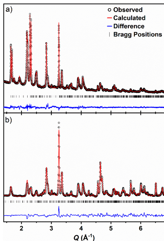
Fig. 4 Rietveld plots of the joint refinements against (a) X-ray ( \lambda = 1.542 Å) and (b) neutron diffraction data ( \lambda = 1.594 Å) in the space group P2_1/a .
