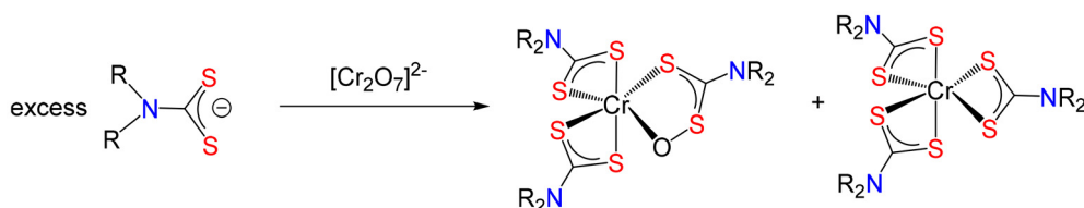
Fig. 24 \text{Cr}(\text{iii}) complexes from reaction of dithiocarbamates and \text{K}_2[\text{Cr}_2\text{O}_7] .
