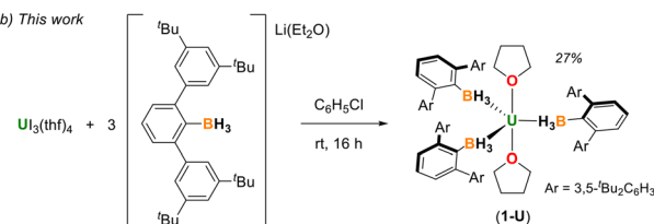
Fig. 1 (a) Notable examples of bulky m -terphenyl ligand scaffolds used to isolate mononuclear uranium complexes. (b) Synthesis of [\text{U}^{\text{III}}(\text{H}_3\text{BAR}^{\text{tBu}_4})_3(\text{thf})_2] ( 1-U ).
