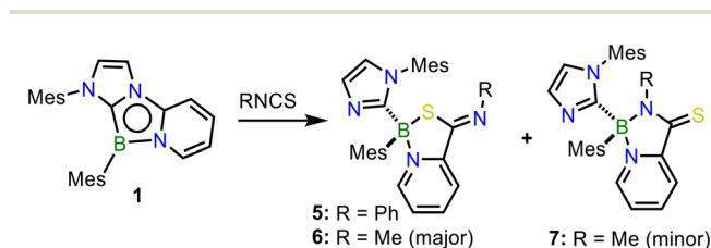
Scheme 3 Reactions of 1 with isothiocyanates.
