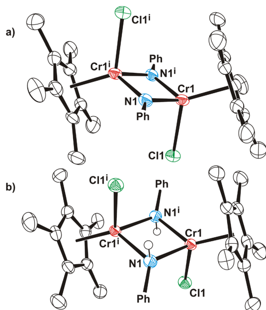
Fig. 1 Perspective views of (a) 2 and (b) 3 ·2C 6 H 5 F with thermal ellipsoids at the 50% probability level. Hydrogen atoms of the η 5 -C 5 Me 5 ligands and phenyl groups are omitted for clarity. The two fluorobenzene solvent molecules in 3 are also omitted. Symmetry code: (i) 1 - x , 1 - y , 1 - z .
