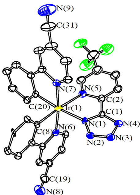
Fig. 1 Molecular structure of [\text{Ir}(\text{ppyCN})_2(\text{PTZ-CF}_3)] with the key atoms labelled. H-atoms have been omitted for clarity. Displacement ellipsoids are at the 30% probability level. Selected bond lengths (Å) and angles ( ^\circ ): Ir(1)–N(1) 2.108(14), Ir(1)–N(5) 2.169(16), Ir(1)–N(6) 2.022(17), Ir(1)–N(7) 2.028(18), Ir(1)–C(8) 2.032(18), Ir(1)–C(20) 2.04(2), C(1)–N(1) 1.33(2), N(1)–N(2) 1.34(2), N(2)–N(3) 1.30(2), N(3)–N(4) 1.35(2), N(4)–C(1) 1.32(3), C(1)–C(2) 1.45(3), C(19)–N(8) 1.15(3), C(31)–N(9) 1.16(4), N(1)–Ir(1)–C(20) 173.9(7), N(7)–Ir(1)–N(6) 172.0(7), N(5)–Ir(1)–C(8) 174.2(7), N(1)–Ir(1)–N(5) 76.2(6), C(1)–N(1)–N(2) 139.6(12), N(1)–N(2)–N(3) 108.6(16), N(2)–N(3)–N(4) 110.8(17), N(3)–N(4)–C(1) 102.9(17), N(1)–C(1)–N(4) 127.2(19).
