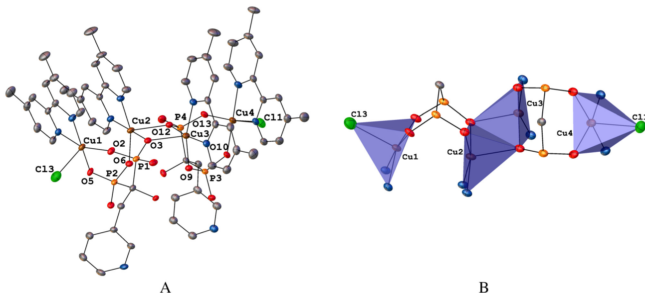
Fig. 1 (A) ORTEP diagram at 40% probability of 1 . Hydrogen atoms and solvent molecules were omitted for clarity. (B) Combined ORTEP/polyhedral representation of the \text{Cu}_4 core from 1 .
