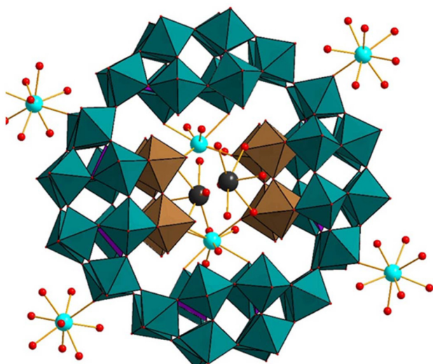
Fig. 18 Combined polyhedral/ball-and-stick representation of [K_{4.5}ClSn]_8P_8W_{48}O_{184}^{17.5-} . Color code: WO_6 octahedra (green), PO_4 tetrahedra (pink), O (red), Sn (brown), K (grey), Cl (green). 129
