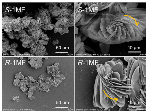
Fig. 2 SEM images of the self-assembled products of \text{In}(\text{NO}_3)_3/\text{S-} , \text{R-pempH}_2 in 90 vol% IPA/ \text{H}_2\text{O} at 100 °C ( S-1MF and R-1MF ).
