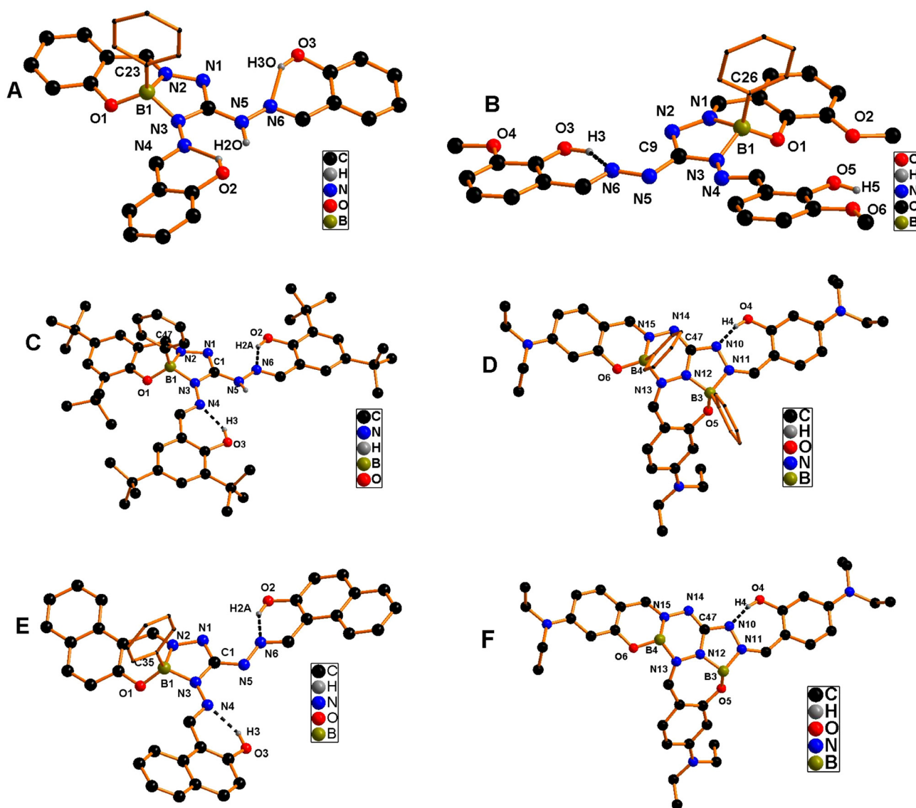
Fig. 1 (A–E) Molecular structure of compounds 6–10. (F) View of boron fused two six membered, one five membered and seven membered heterocycles of compound 9, here phenyl group on boron atoms are omitted for clarity.
