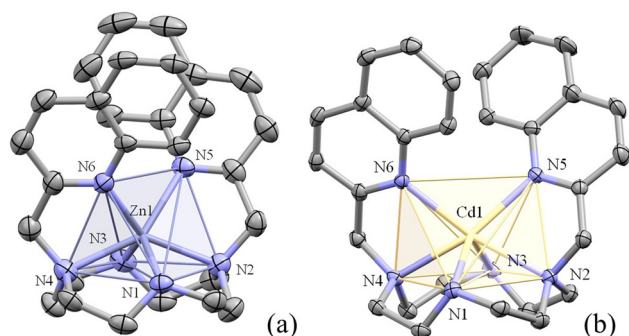
Fig. 2 Coordination geometry and labelling scheme for [ZnL3] 2+ (a) and [CdL3] 2+ (b) complexes, showing similar distorted trigonal prism coordination environments. Ellipsoids drawn at the 50% probability level. Hydrogen atoms are omitted for clarity.
