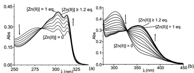
Fig. 8 UV-vis spectra of L3 (a) and HL2 (b) in aqueous solutions at pH 7 in the presence of increasing amounts of Zn(II) ([L3] = 6 \times 10^{-6} M, [HL2] = 5.2 \times 10^{-5} ).
