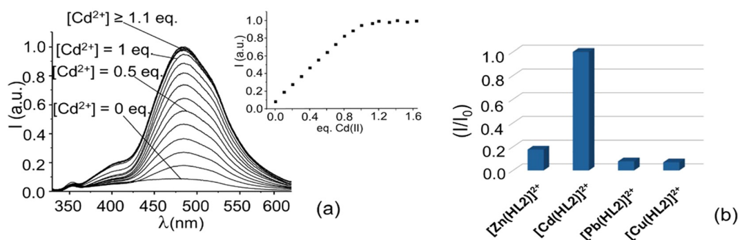
Fig. 10 Emission spectra of HL2 in the presence of increasing amounts of \text{Cd(II)} (inset: emission intensity at 484 nm as a function of \text{Cd(II)} equivalents added) (a) and comparison of the emission intensity of the complexes with HL2 in the presence of 1 equivalent of \text{Zn(II)} , \text{Cd(II)} , \text{Pb(II)} and \text{Cu(II)} (the I/I_0 values are normalized to the emission of the \text{Cd(II)} complex, taken equal to 1) (b) ( [\text{HL2}] = 9.5 \times 10^{-6} \text{ M} , \lambda_{\text{exc}} = 320 \text{ nm} ).
