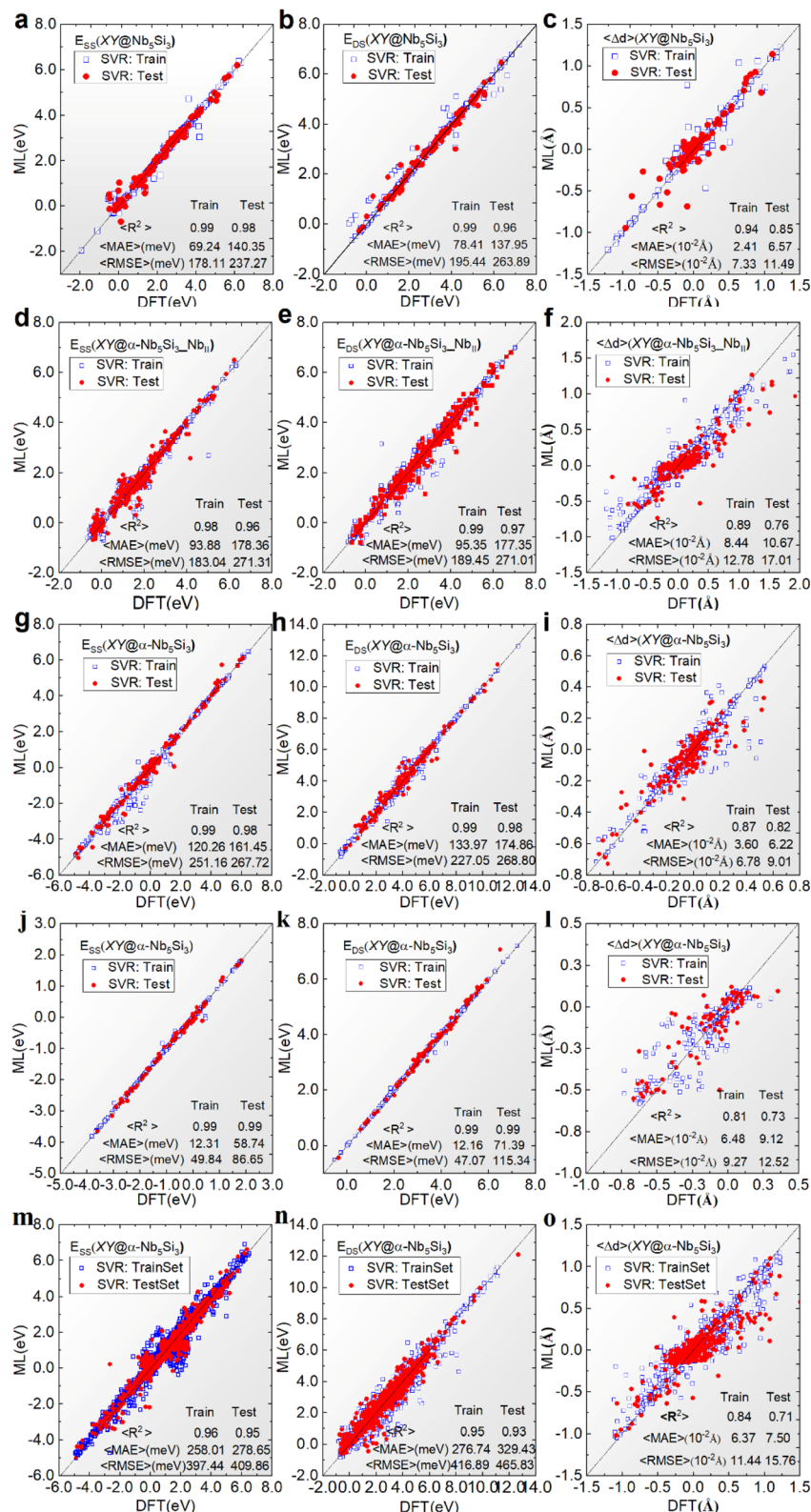
Fig. 4 E_{SS} , E_{DS} , and \langle \Delta d \rangle of the \alpha\text{-Nb}_5\text{Si}_3 substitution systems at the four non-equivalent sites (a–c) \text{Nb}_i , (d–f) \text{Nb}_{II} , (g–i) \text{Si}_i , (j–l) \text{Si}_{II} , and (m–o) all sites predicted by the \text{CE}_{\text{AET}}\text{-SVR} models compared with the DFT results.
