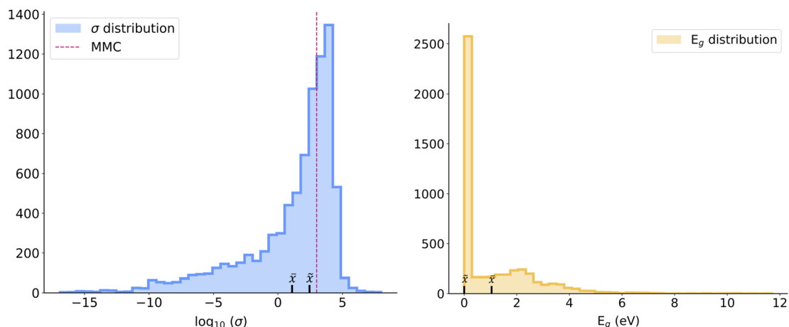
Fig. 1 Data distributions for \sigma (left) and E_g (right). \bar{x} and \hat{x} denote the mean and the median, respectively. The purple dotted line on \sigma distribution indicates the minimum metallic conductivity \sigma_{\min} = 10^3 (S cm ^{-1} ).
