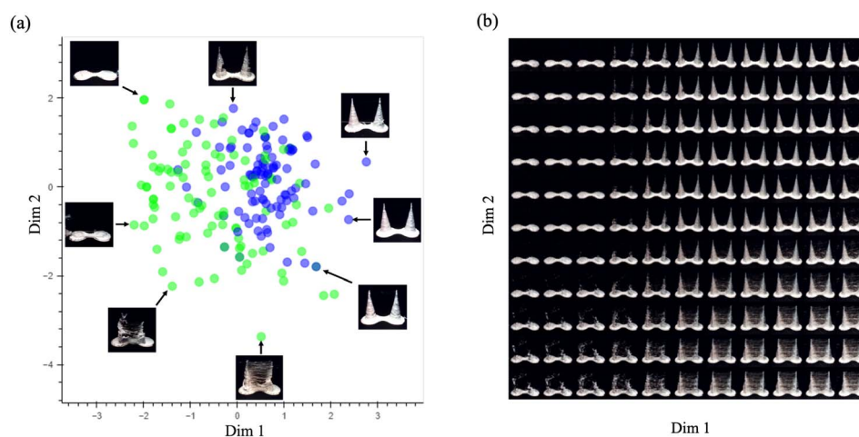
Fig. 10 Feature analysis of the cone VAE. (a) The location of preferred (purple) and dis-preferred (green) vases in a two-dimensional projection of the 8-dimensional feature space. Image insets are VAE-generated synthetic cones at the indicated locations. (b) The same 2D projection as in (a), but filled with VAE-generated synthetic cones to clarify the features visible in this condensed view of the feature space.
