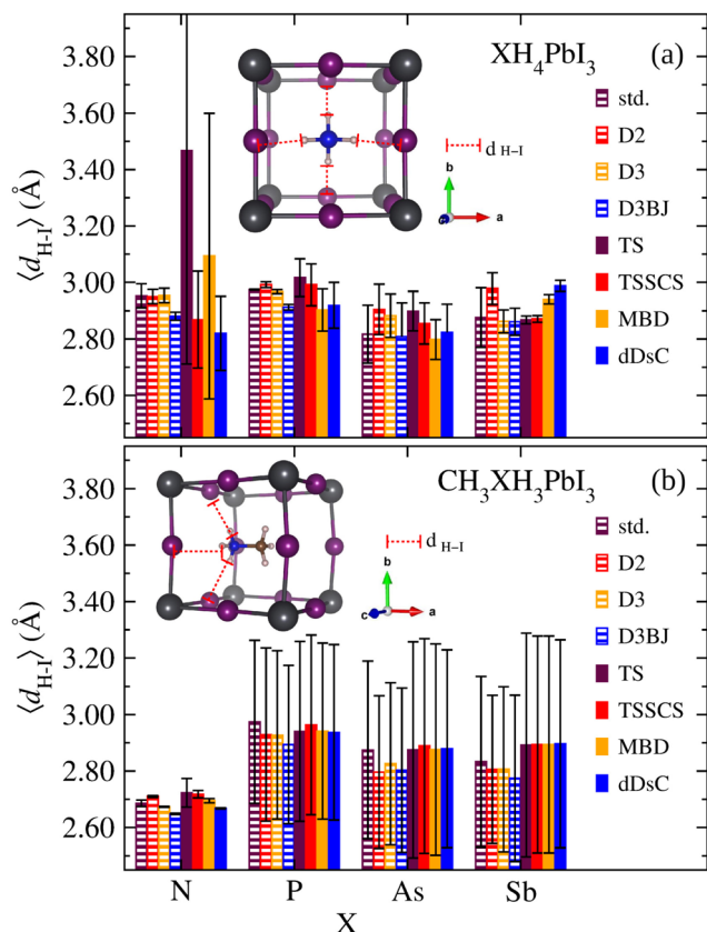
Fig. 5 The average H–I bond lengths, \langle d_{H-I} \rangle , considering the H atoms bonded to the X atoms, for (a) \text{XH}_4\text{PbI}_3 and (b) \text{CH}_3\text{XH}_3\text{PbI}_3 as a function of X (X = N, P, As, and Sb) for calculations without vdW (std) and with empirical (D2, D3, and D3BJ) or semi-empirical (TS, TSSCS, MBD, and dDsC) vdW corrections. The bars corresponding to the mean squared deviation are indicated for each system and its respective calculation method.
