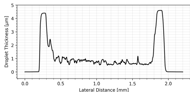
(b) Cs 3 Bi 2 Br 9 -Cs 3 Sb 2 I 9 Droplet Thickness Profile
