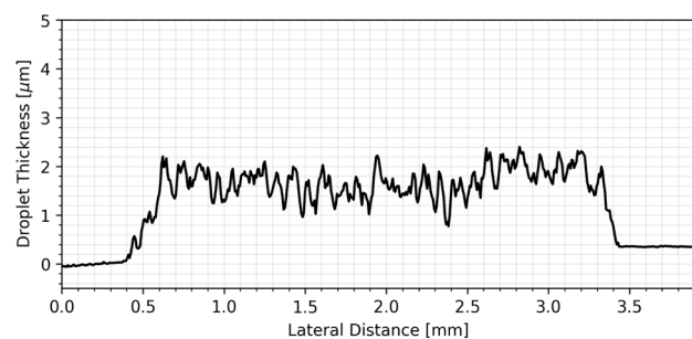
(a) FAPbI 3 -MAPbI 3 Droplet Thickness Profile
