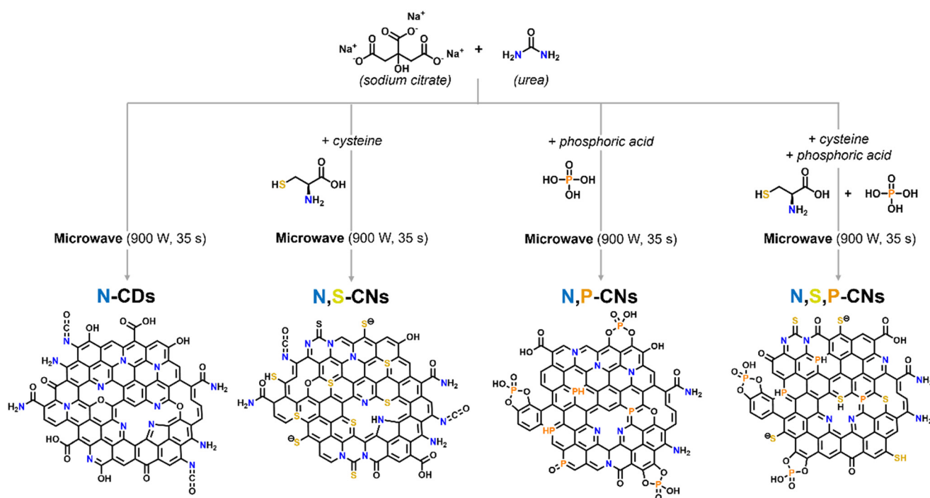
Scheme 1 Methodology for the synthesis of the multi-doped carbon nanomaterials: N-CDs; N,S-CN; N,P-CN; and N,S,P-CN.
