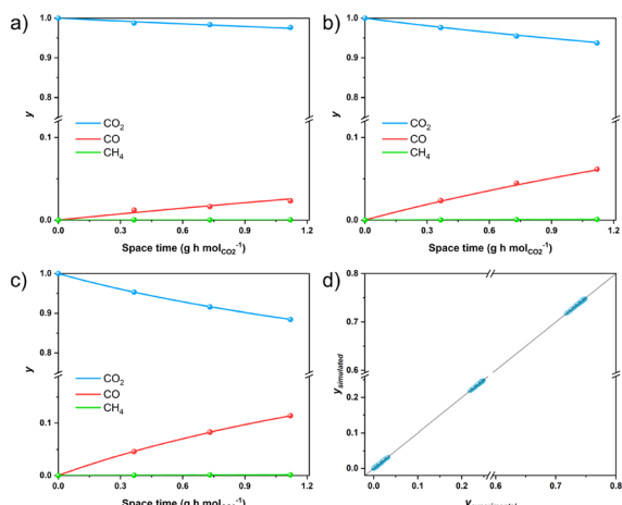
Fig. 5 Experimental data fitting of the \text{CO}_2 hydrogenation reaction over the FeTi@C550-5 catalyst at 30 bar, \text{H}_2/\text{CO}_2 = 3 and at a) 375 °C, b) 400 °C and c) 425 °C. d) Parity plot of the calculated and experimental molar fractions.
