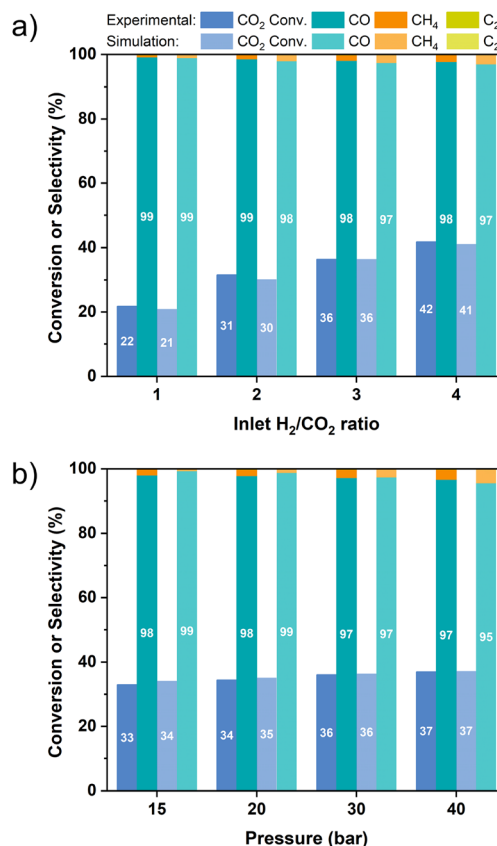
Fig. 6 Aspen simulation results using the estimated kinetic parameters compared with the experimental catalytic data on FeTi@C550-5 at different a) feed ratios at P = 30 bar and b) pressures at \text{H}_2/\text{CO}_2 = 3 . Conditions: T = 425 °C, GHSV = 12 000 \text{mL g}_{\text{cat}}^{-1} \text{h}^{-1} .
