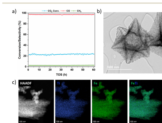
Fig. 4 a) Stability test over 60 hours of operation. CO 2 conversion (blue) and CO (red) and CH 4 (green) selectivity values of the hydrogenation of CO 2 over FeTi@C550-5. Reaction conditions: H 2 /CO 2 = 3, T = 425 °C, P = 30 bar, GHSV = 64 000 mL g cat −1 h −1 . b) TEM image and c) elemental mapping by STEM-EDX of FeTi@C550-5 after 60 h on stream.
