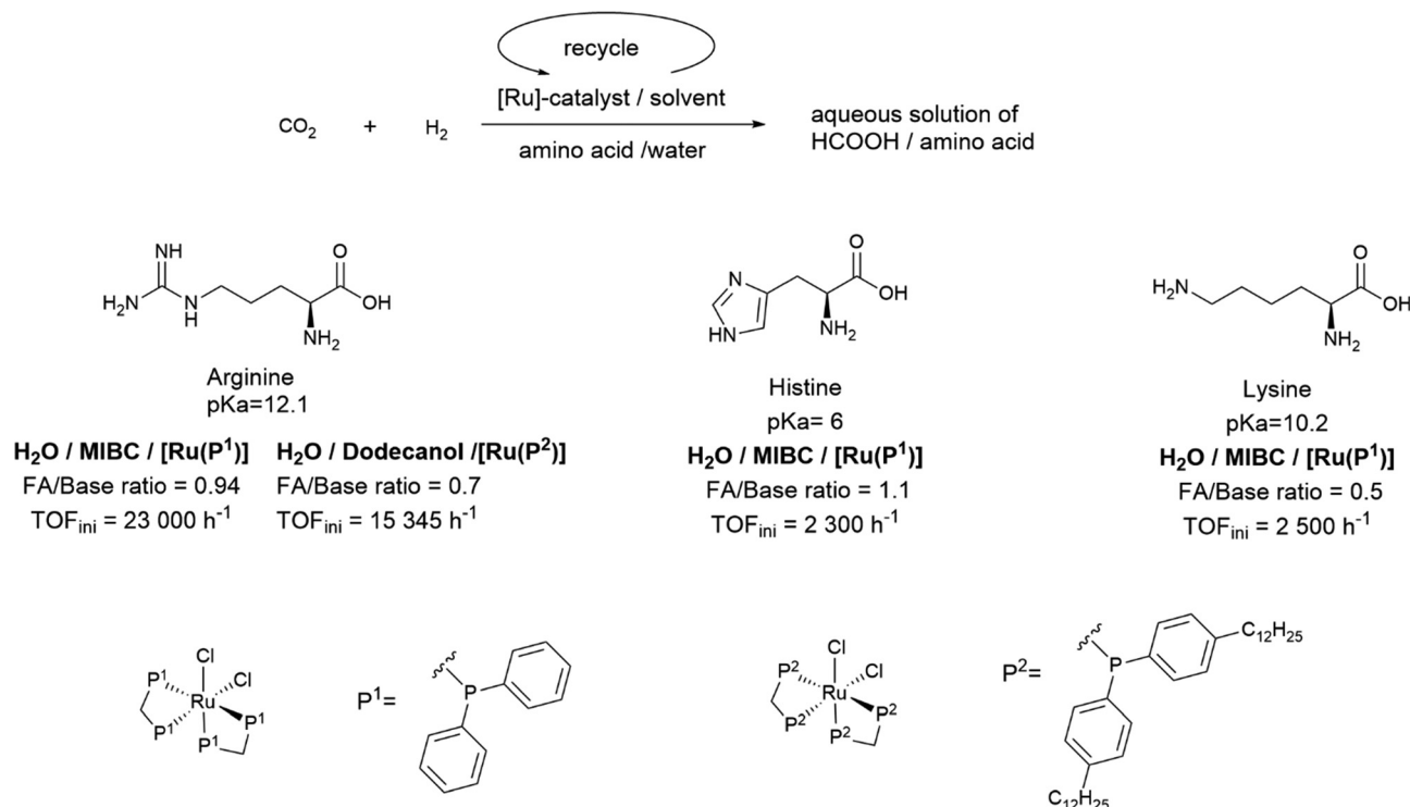
Fig. 15 The reaction system for the CO 2 hydrogenation to product HCOOH/amino acids mixture as the animal feeds additive using a biphasic system with cis -[Ru(dpppm) 2 Cl 2 ] (P 1 ligand) and cis -[Ru(C 12 -dpppm) 2 Cl 2 ] (P 2 ligand) catalysts. MIBC, methyl isobutyl carbinol. Reproduced from ref. 124 with copyright permission.
