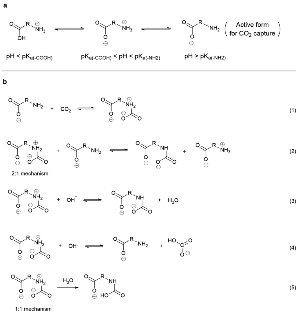
Scheme 2 (a) The dependence of aqueous amino acid form on the pH; (b) possible reactions for \text{CO}_2 capture with active amino acid absorbents.
