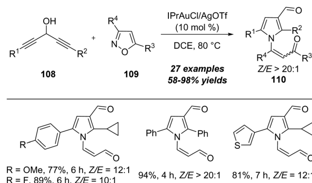
Scheme 36 Gold-catalyzed [4+1] annulation between 1,4-diyne-3-ols 108 and isoxazoles 109 .
