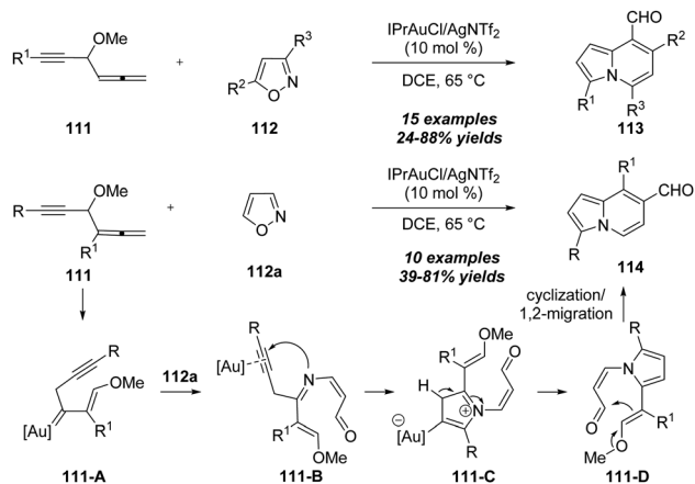
Scheme 37 Gold-catalyzed bicyclic annulations of 4-methoxy-1,2-dienyl-5-yne 111 with isoxazoles 112 .
