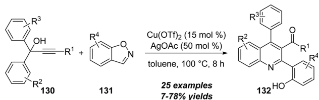
Scheme 42 Copper-catalyzed [4+2] annulation of propargylic alcohols 130 and benzod[1,2]isoxazoles 131 .
