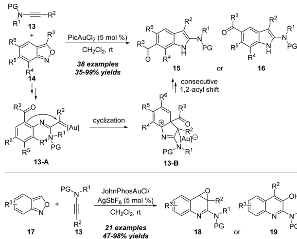
Scheme 6 Gold-catalyzed formal [3+2] annulation of ynamides 13 with anthranils 14 or 17 .
