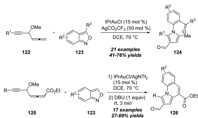
Scheme 40 Gold-catalyzed [4+1] annulation of 4-methoxy-1,2-dienyl-5-yne 122 or 125 with anthranils 123 .
