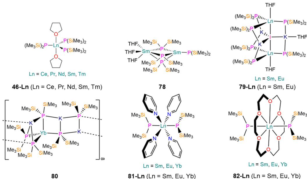
Fig. 23 Ln(II) complexes [Ln(P '' ) 3 (THF) 2 ] ( 46-Ln ; Ln = Ce, Pr, Nd, Sm, Tm), [Sm(P '' )(μ-P '' ) 3 Sm(THF) 3 ] ( 78 ), [(Ln(P '' ) 3 (THF)) 2 (μ-I)K 3 (THF)] ( 79-Ln ; Ln = Sm, Eu), [KYb(P '' ) 3 {μ-K(P '' ) 2 }] ∞ ( 80 ), trans -[Ln(P '' ) 2 (py) 4 ] ( 81-Ln ; Ln = Sm, Eu, Yb), [Ln(P '' ) 2 (18-crown-6)] ( 82-Ln ; Ln = Sm, Eu, Yb).
