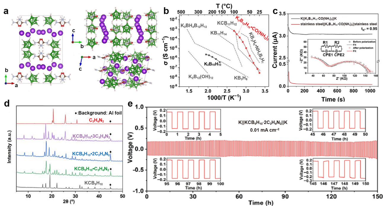
Fig. 42 (a) Crystal structure of K_2B_{10}H_{10} \cdot CO(NH_2)_2 . (b) Temperature dependence of the solid-state K-ion conductivity. (c) Chronoamperometric curves of the K||K_2B_{10}H_{10} \cdot CO(NH_2)_2||K and stainless steel ||K_2B_{10}H_{10} \cdot CO(NH_2)_2|| stainless steel cells at a polarized voltage of 0.5 V. The inset shows Nyquist plots of a K||K cell before and after polarization. Reproduced with permission from ref. 306. Copyright 2024, American Chemical Society. (d) XRD patterns of KCB_9H_9 , C_3H_4N_2 , and KCB_9H_9 \cdot nC_3H_4N_2 ( n = 1, 2 , and 3). (e) Voltage profiles of the K||K symmetric cell at room temperature and 0.01 mA\ cm^{-2} . Reproduced with permission from ref. 307. Copyright 2024, Wiley-VCH.
