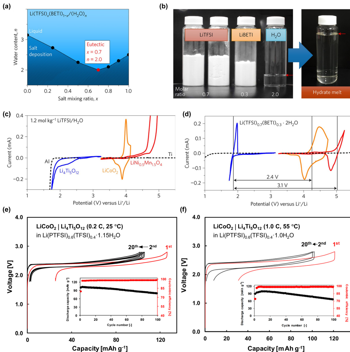
Fig. 7 (a) and (b) Preparation of dihydrate melt by exploring the eutectic point of \text{Li}(\text{TFSI})_x(\text{BETI})_{1-x} salt/water mixtures. (c) and (d) Cyclic voltammograms of \text{Li}_4\text{Ti}_5\text{O}_{12} , \text{LiCoO}_2 , \text{LiNi}_{0.5}\text{Mn}_{1.5}\text{O}_4 electrodes in \text{Li}(\text{TFSI})_{0.7}(\text{BETI})_{0.3}\cdot 2\text{H}_2\text{O} . 19 (e) and (f) Electrochemical performance of aqueous \text{LiCoO}_2|\text{Li}_4\text{Ti}_5\text{O}_{12} full cells in the monohydrate-melt \text{Li}(\text{PTFSI})_{0.6}(\text{TFSI})_{0.4}\cdot 1\text{H}_2\text{O} electrolyte. 85 Reprinted with permission from Nature Energy and Electrochemistry Communications .
