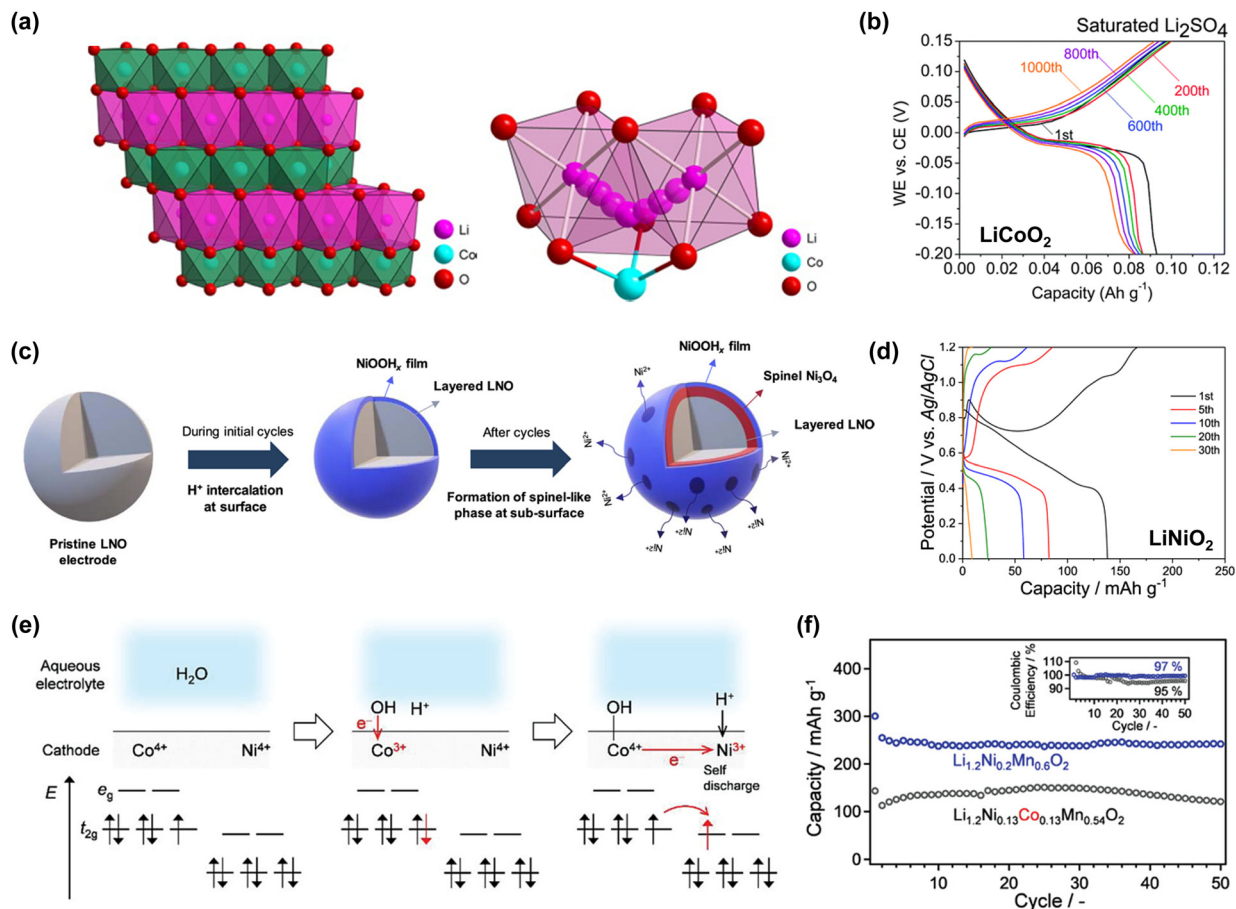
Fig. 22 (a) Crystal structure and Li + diffusion pathway in layered LiCoO 2 . 268 (b) Long-term cycling of LiCoO 2 in a sat. Li 2 SO 4 solution. 273 (c) Degradation mechanism of LiNiO 2 in the aqueous electrolyte. 274 (d) Charge/discharge curves of LiNiO 2 in 1.0 M LiNO 3 /H 2 O. 274 (e) Schematic of the self-discharge process in the Co-doped layered oxide, Li 1.2 Ni 0.13 Co 0.13 Mn 0.54 O 2 . 275 (f) Cycling stability of Li 1.2 Ni 0.2 Mn 0.6 O 2 and Li 1.2 Ni 0.13 Co 0.13 Mn 0.54 O 2 in the dihydrate melt, Li(TFSI) 0.7 (BETI) 0.3 ·2H 2 O. 275 Reprinted with permission from Progress in Natural Science: Materials International (a), Energy & Environmental Science (b), ACS Applied Materials & Interfaces (c), and Advanced Science (d).
