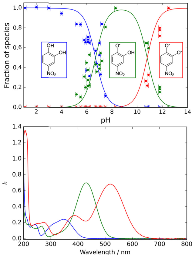
Fig. 7 Upper panel: pH-Dependent fractions of 4-nitrocatechol (4NC), singly deprotonated ( 4\text{NC}^- ), and doubly deprotonated ( 4\text{NC}^{2-} ) ions. Data points represent experimental values obtained via UV/visible spectroscopy, while the lines correspond to equilibrium calculations based on literature-reported \text{pK}_a values. Lower panel: Wavelength-dependent imaginary refractive indices for individual 4NC, 4\text{NC}^- , and 4\text{NC}^{2-} species, highlighting their distinct optical absorption characteristics. Reproduced from ref. 155 with permission from the American Chemical Society, copyright 2024.
