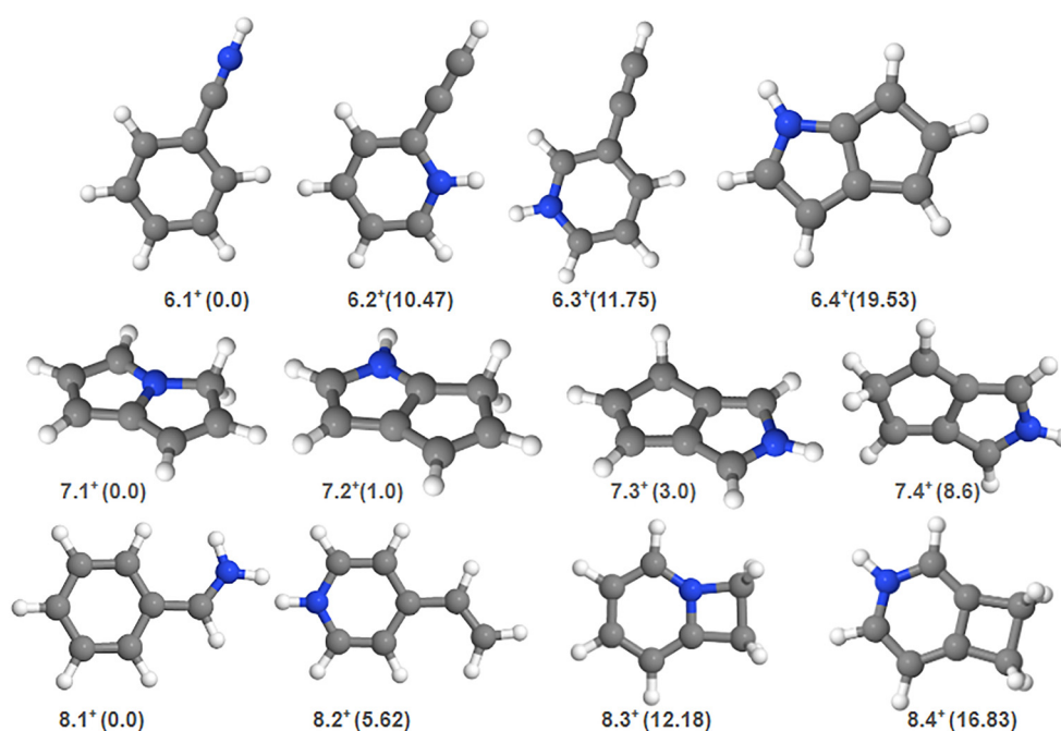
Fig. 9 Low-energy isomers of \text{C}_6\text{H}_5\text{CNH}^+ ( m/z = 104 ) (top), \text{C}_6\text{H}_5\text{CHNH}^+ ( m/z = 105 ) (middle) and \text{C}_6\text{H}_5\text{CHNH}_2^+ ( m/z = 106 ) (bottom), obtained with the ABCluster software combined with DFT computations. Carbon atoms are gray, hydrogen atoms are white and nitrogen atoms are blue. The numbers in parentheses are the relative energies in \text{kcal mol}^{-1} obtained at the CCSD(T)/cc-pVTZ level of theory. Energy parameters and T1 diagnostics for CCSD(T) are shown in Tables S10–S12 (SI). For details about CASSCF/NEVPT2/def2-TZVP energies and active space orbitals, see Table S11 and Fig. S12–S15 in the SI.
