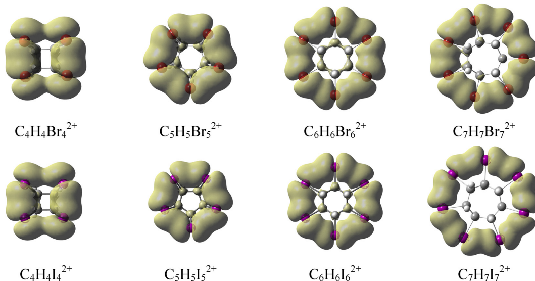
Fig. 8 Top view of the \sigma -EDDB H function isosurfaces (isovalve: 0.001 a.u.) for dicationic halogenated cycloalkanes.
