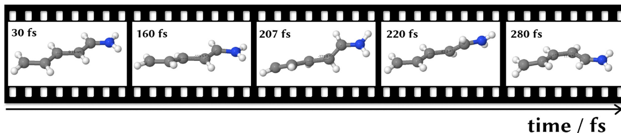
Fig. 7 Average structure of PSB3 (averaged over the 20 Gaussian centers with a weight proportional to the amplitude of each Gaussian in the linear combination – A_i , in eqn (1) –) for the DD-vMCG/20GWP propagation, showing how trans -PSB3 isomerises to cis -PSB3 in 300 fs.
