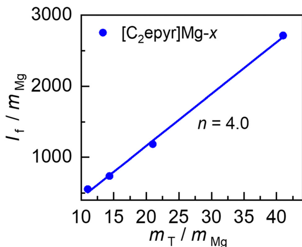
Fig. 3 Plots of I_f/m_{Mg} versus m_T/m_{Mg} for the 1220\text{ cm}^{-1} band of [C_2\text{epyr}]\text{Mg}-x . n : solvation number.
