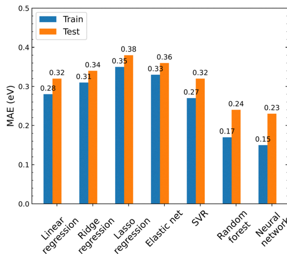
Fig. 2 Training and test prediction accuracy (mean absolute error – MAE) of different MLAs for predicting U_{\text{limiting}} of the NRR at the surface of bimetallic alloy catalysts.
