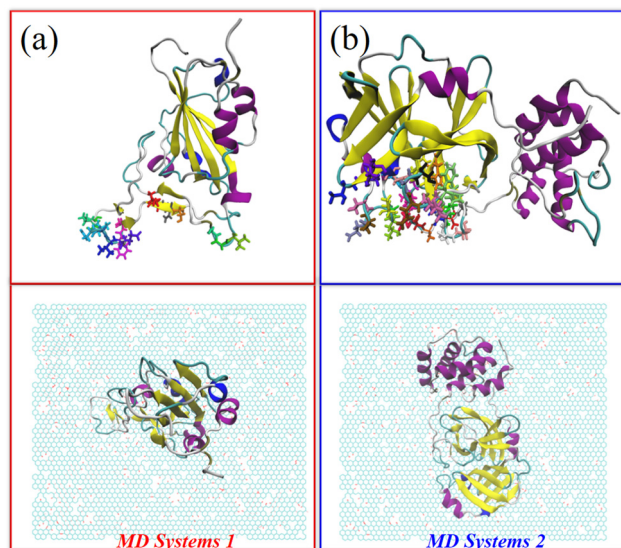
Fig. 1 From the top views, (a) the MD systems for the RBD-investigated materials and (b) M^{\text{Pro}} -investigated materials. The conformation of proteins and investigated materials at the initial input stage, i.e. , at 0 ns. RBD and M^{\text{Pro}} highlighted by “Newcartoon” drawing methods. Three important contact regions (CR1–CR3) for the RBD and active pocket of M^{\text{Pro}} highlighted by “Licorice” drawing methods. The C, O, H and F atoms of the investigated materials are represented by cyan, red, white and pink balls, respectively. Water molecules are hidden for clarity.
