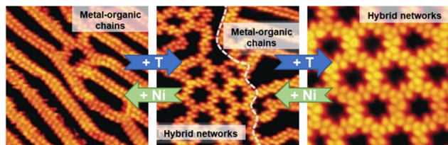
Fig. 9 Reversible structural transformation of Ni-based metal-organic nanostructures on Au(111) in response to additional T molecules or Ni atoms. Reproduced with permission. 139 Copyright 2016 WILEY-VCH Verlag GmbH & Co. KGaA, Weinheim.
