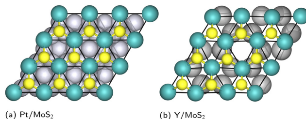
Fig. 4 Structures of the \text{Pt}/\text{MoS}_2 and \text{Y}/\text{MoS}_2 interfaces. Mo: cyan; S: grey; Pt silver; Y: grey.
