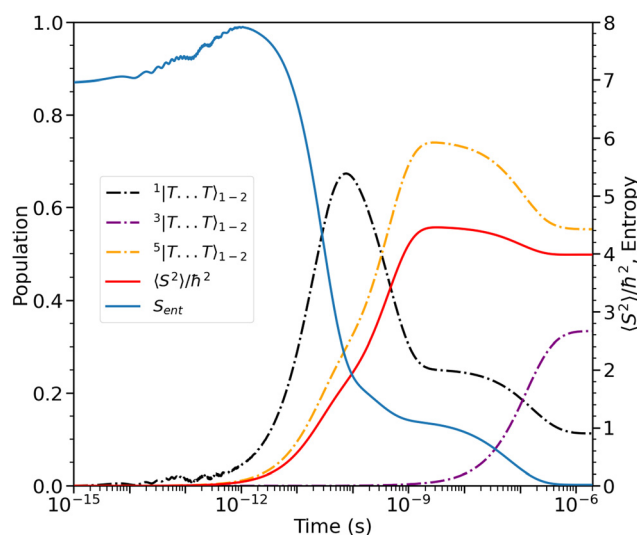
Fig. 8 The entanglement entropy, S_{\text{ent}} , and expectation value of the spin, \langle S^2 \rangle . The populations of the interchain triplet-pair states are also shown. Once the system reaches thermal equilibrium at ca. 2 \mu\text{s} the values of the entropy and \langle S^2 \rangle are approximately 0 and 4h^2 , respectively, corresponding to complete singlet fission to a pair of unentangled triplets. We see that this is equivalent to equal populations of the triplet-pair states, i.e. , P(^1|T \cdots T)_{1-2} = \frac{1}{9} , P(^3|T \cdots T)_{1-2} = \frac{3}{9} and P(^5|T \cdots T)_{1-2} = \frac{5}{9} .
