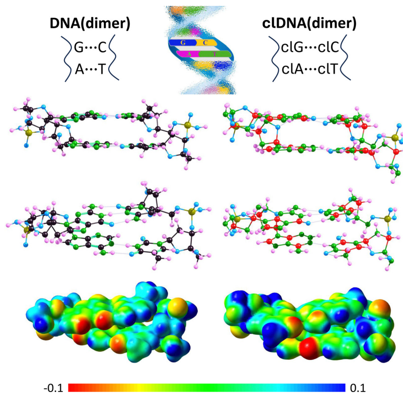
Fig. 9 Equilibrium structures (determined at the \omega B97XD/aug-cc-pVDZ theory level) of DNA(dimer) containing A–T and G–C complementary pairs (left panel) and cDNA(dimer) containing cA–cT and cG–cC carbonless base pairs (right panel), each depicted in two views. The corresponding molecular electrostatic potential (MEP) maps calculated based on \omega B97XD/aug-cc-pVDZ electron densities and plotted on the 0.01 a.u. isodensity surface are presented below. The values on the electrostatic potential scale are presented in atomic units (a.u.).
