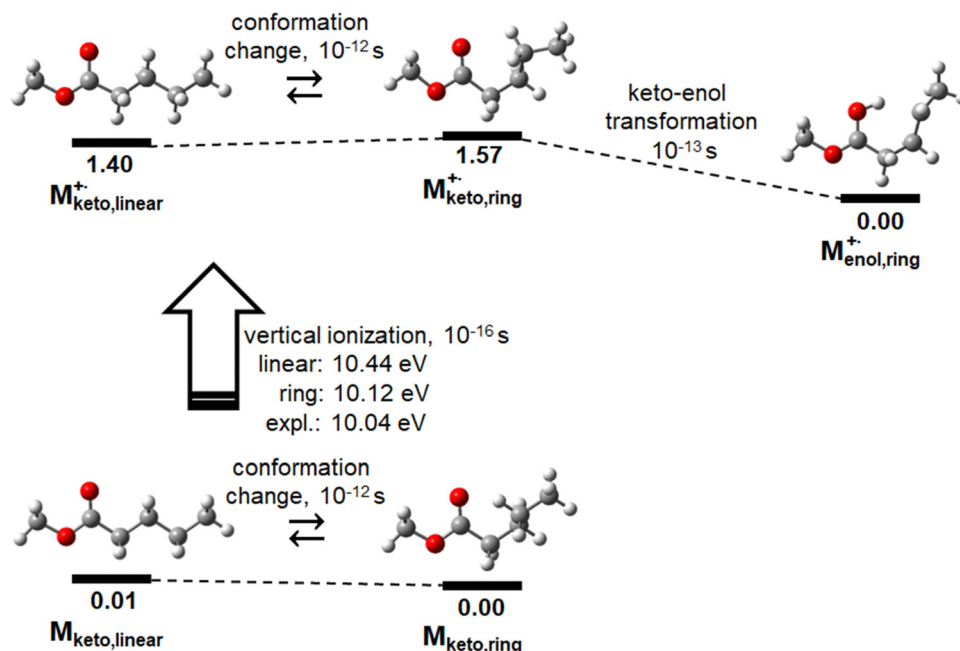
Fig. 5 The energy profile in eV for the conformational change of the neutral molecule M and the molecular ion M^+ and the keto–enol transformation at the M06-2X/6-31+G(d) level of theory.
