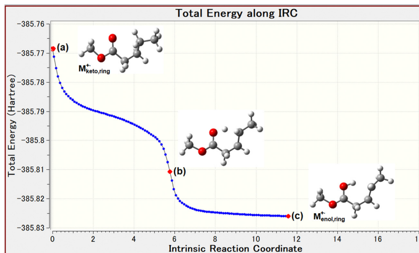
Fig. 6 Intrinsic reaction coordinate (IRC) for (a) keto to (c) enol transformation of the molecular ion M^+ of methyl valerate. Points a, b, and c represent the start, inflection, and end points, respectively.
