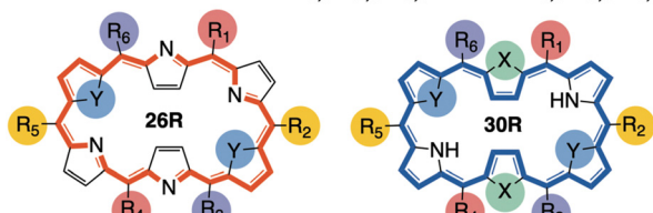
Substitution Pattern: \text{NH}_2\text{Y}_2\text{R}_{1,4}\text{R}_{2,5}\text{R}_{3,6} and \text{X}_2\text{Y}_2\text{R}_{1,4}\text{R}_{2,5}\text{R}_{3,6}
