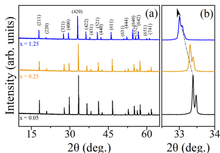
Fig. 5 (a) Room temperature powder X-ray diffraction patterns of \text{Y}_3-\text{Al}_{5-x}\text{Sc}_x\text{O}_{12} garnet x = 0.05, 0.25 , and 1.25 . (b) Magnified view of peak shifting to low 2\theta side with increasing x .
